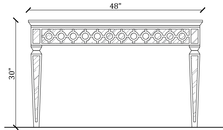
FRONT VIEW WOODEN CONSOLE
